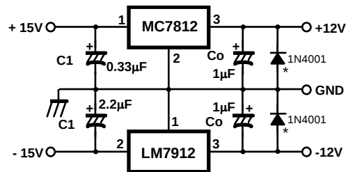
Figure 7. Split power supply ( \pm 12V/1A )
